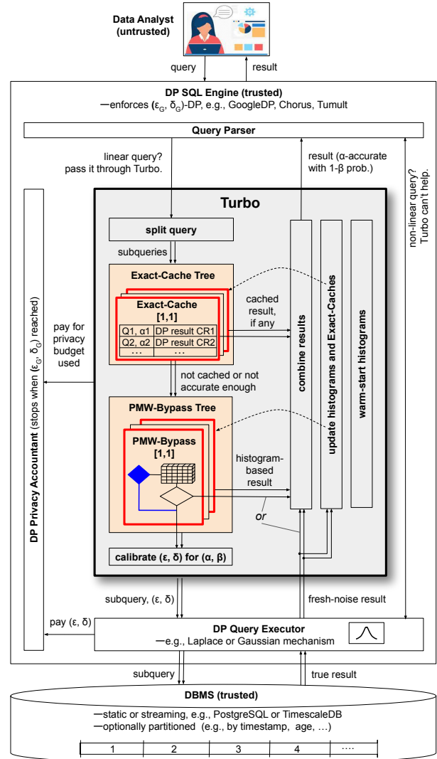
Fig. 1. Turbo architecture.
